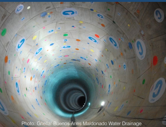
Photo: Ghella: Buenos Aires Maldonado Water Drainage
